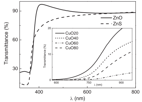
Fig. 4. Optical transmittance spectra of ZnO, ZnS and CuO thin films at various thickness in inset.
