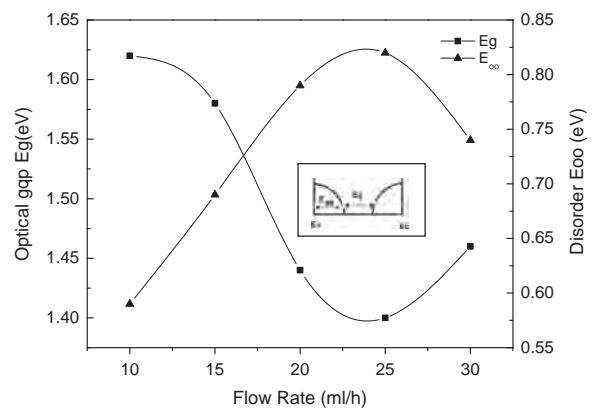
Fig. 8. Variation of the optical band gap and disorder in film network as a function of the flow rate. Inset figure is a schematic drawn of energy band diagram.
