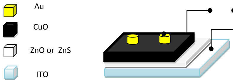
Figure II. 21 A schematic cross section of the produced solar cells.
