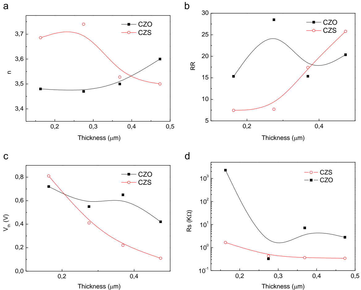
Fig. 6. Variation of heterojunction parameters vs. thickness: (a) Ideality factor ( n ), (b) Rectification Ratio (RR), (c) Turn on voltage ( V_{th} ) and (d) Series resistance ( R_s ).
