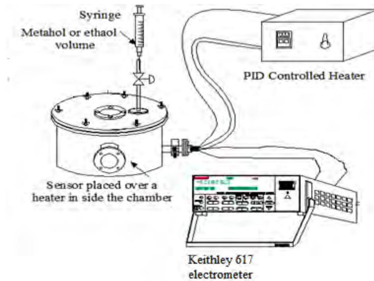
Figure II.18 A schematic diagram of the gas system measurement for organic vapor.
