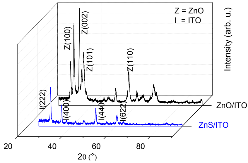
Figure IV.23-a XRD diffraction patterns of ZnO and ZnS films deposited on ITO glass at 300°C.
