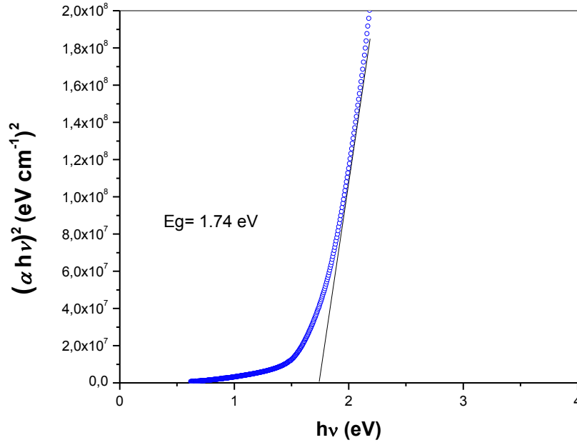
Figure II.10 Typical variation of the quantity (\alpha hv)^2 as a function of photon energy, for the sample prepared with 0.01 M used for the determination of the optical gap.
