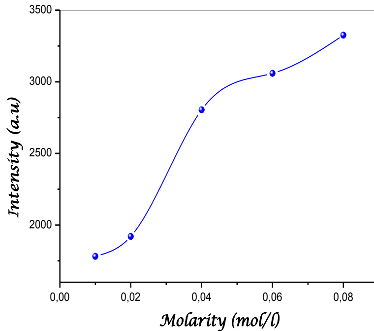
Figure III.30 Variation of Ag Raman mode intensity for CuO films deposited with different molarities.
