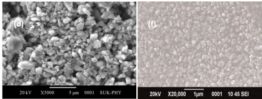
Figure I.2 SEM images of CuO thin films deposited by (a.1 and 2) sputtering, (b) thermal evaporation, (c) SILAR method, (d) sol-gel method, (f) spray pyrolysis [11-26].
