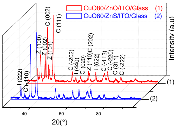
Fig. 3. XRD patterns of CuO80/ZnO and CuO80/ZnS heterojunction deposited onto ITO substrate (C=CuO, Z=ZnO, I= ITO).
