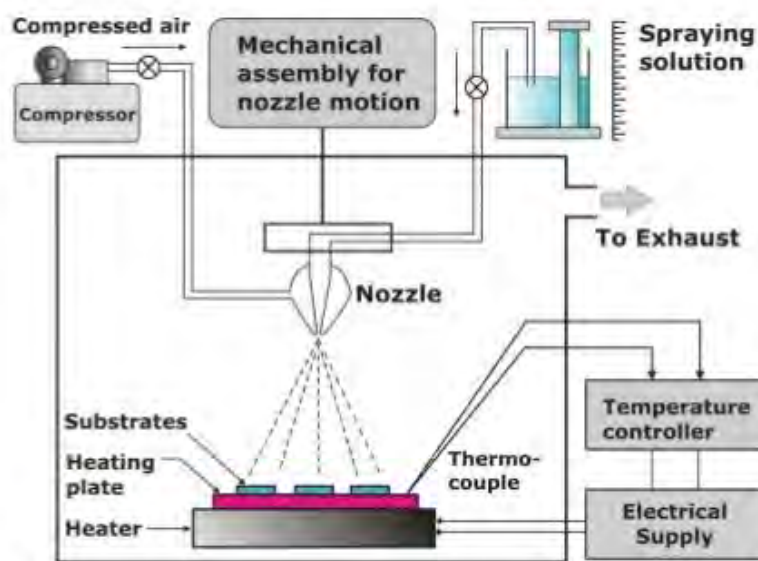
Figure II.4 Schematic set-up for spray pyrolysis technique.
