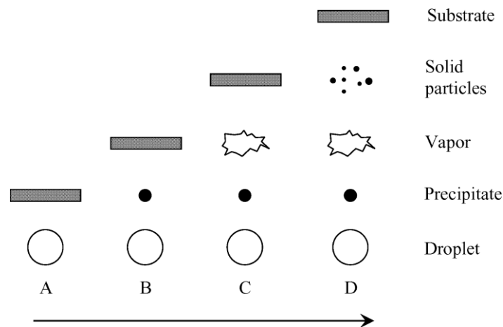
Figure II.6 Description of the deposition processes initiated with increasing substrate temperature.
