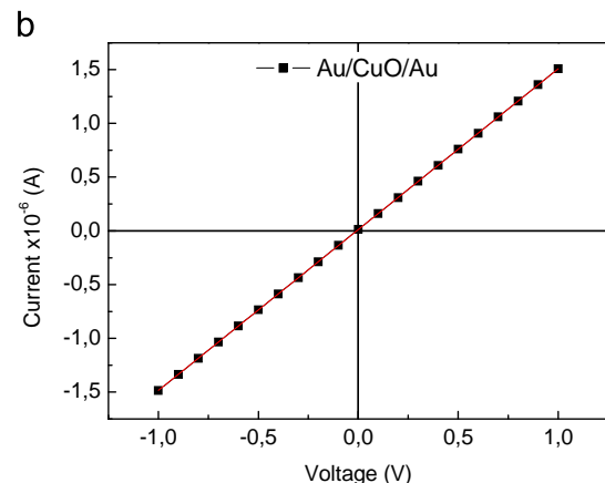
Fig. 1. (a) Schematic structure of Au/p-CuO/n-ZnO (ZnS) hetero-structure, (b) I – V characteristic of Au/CuO/Au structure.
