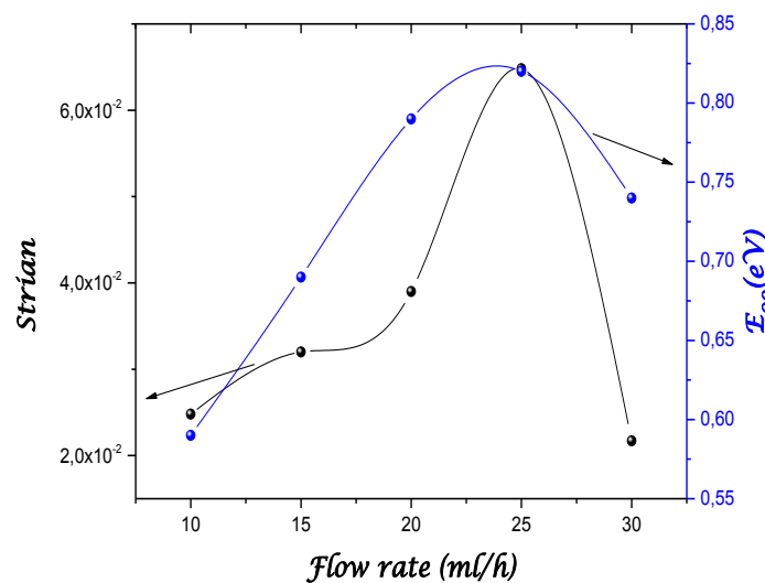
Figure III.48 Variation of strain and disorder in films versus flow rate.
