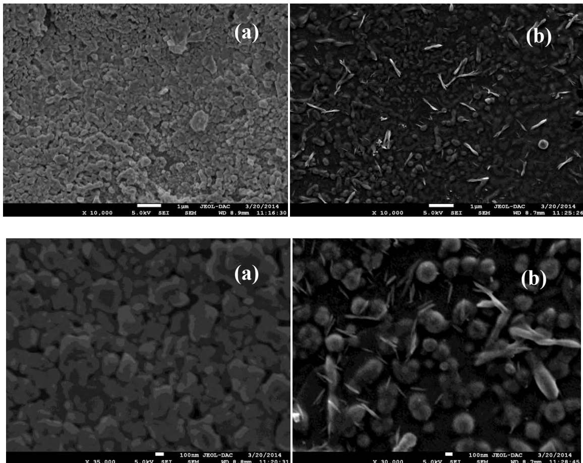
Figure III.55 typical SEM images of CuO films deposited using different of Cu salt source (a) copper chloride and (b) copper acetate.
