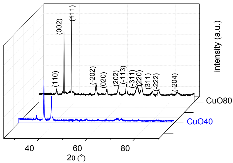
Figure IV.23-b XRD diffraction patterns of CuO films prepared at 300°C.
