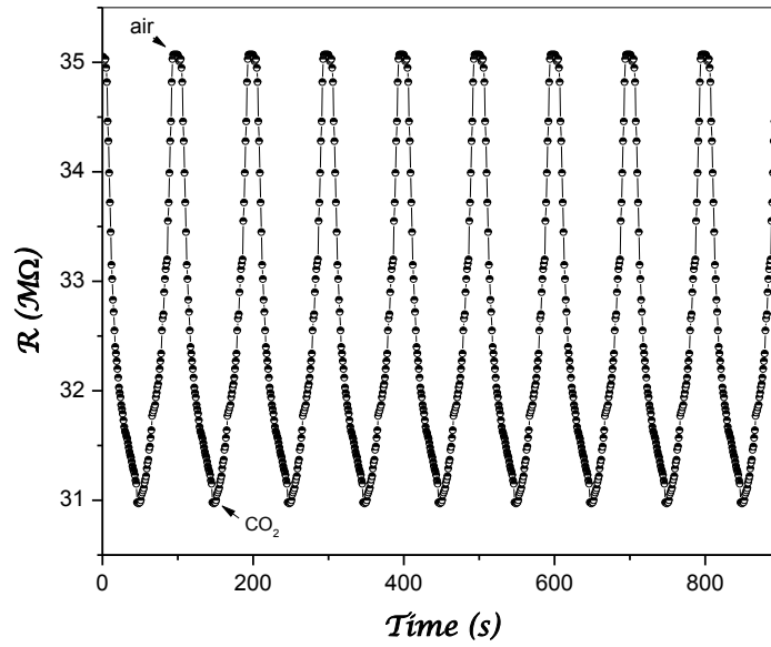
Figure IV.19 Transient resistance of CuO thin film deposited on screen printed gold electrodes. P_{air} = 2 \times 10 \text{ hPa} and P_{CO_2} = 5 \text{ hPa} at 60^\circ\text{C} .
