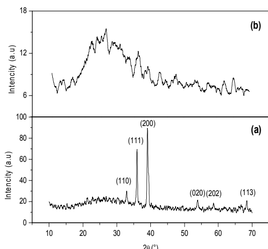
Fig. 1 XRD spectra of \text{CuO} thin films deposited at substrate temperature equal to 300^\circ\text{C} with different solutions: (a) Copper chloride and (b) Copper acetate
