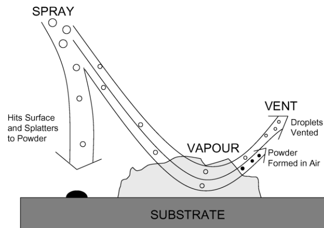
Figure II.5 Aerosol transport.
