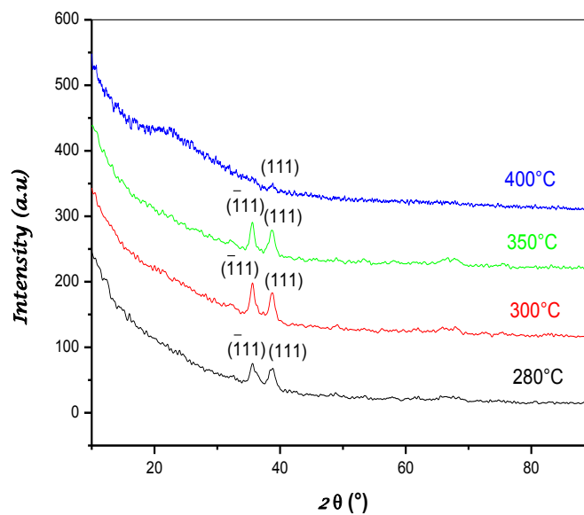
Figure III.16 XRD diffraction patterns of CuO films prepared with different substrate temperatures.
