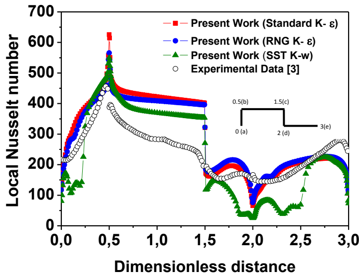
FIGURE 2. Distribution of local Nusselt number for Re_D = 94000 with experimental data.
