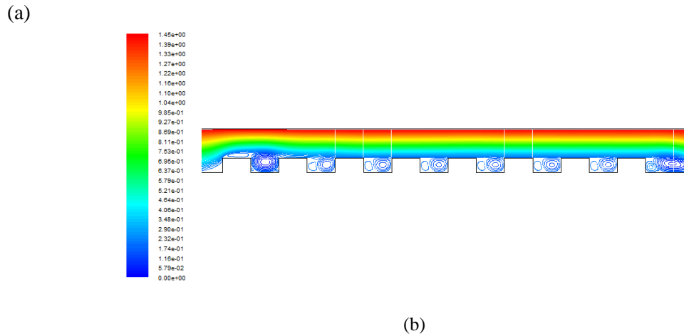
FIGURE 3. Streamlines of the turbulent flow at Re= 9.4 \times 10^4 : (a) Standard k-\epsilon and (b) SST k-\omega
