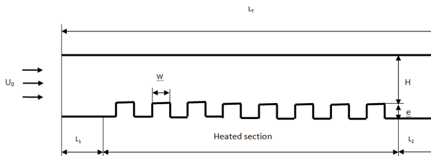
FIGURE 1. Geometry of the present problem
