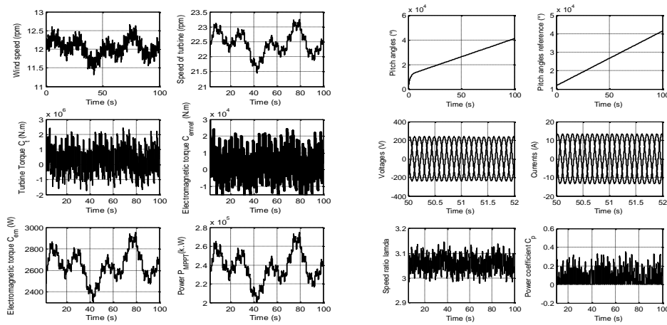
Figure 8. Simulation of a variable speed wind turbine under a high wind and P_{ref} = 150 \text{ kW} .
