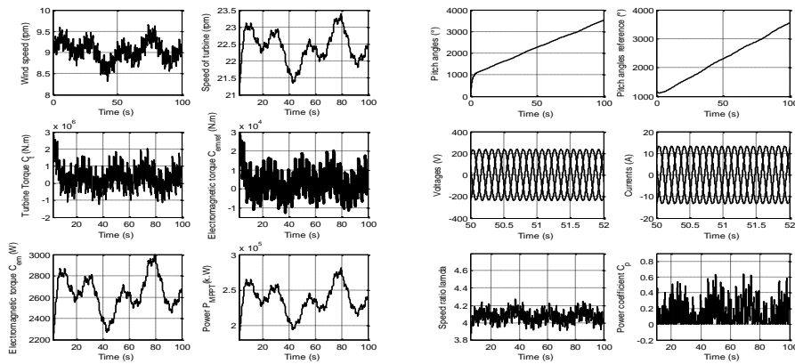
Figure 5. Simulation of a variable speed wind turbine under a medium wind and P_{ref} = 15 kW.
