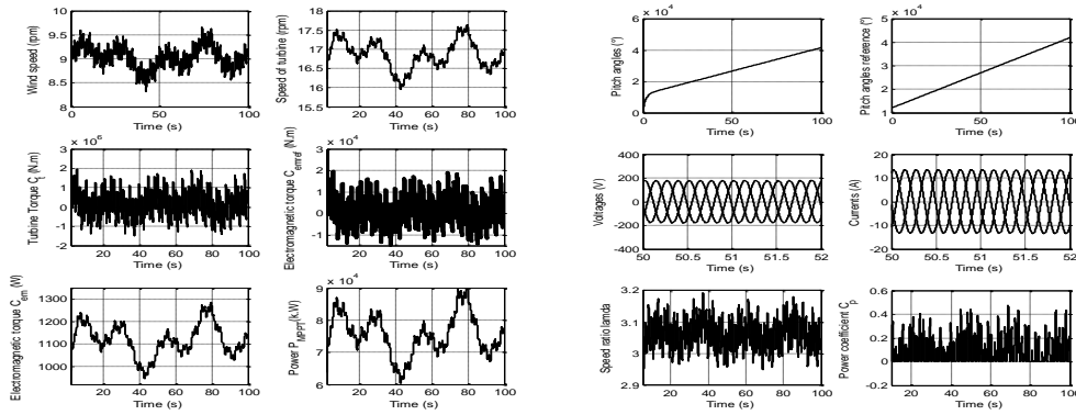
Figure 7. Simulation of a variable speed wind turbine under a medium wind and P_{ref} = 150 \text{ kW} .
