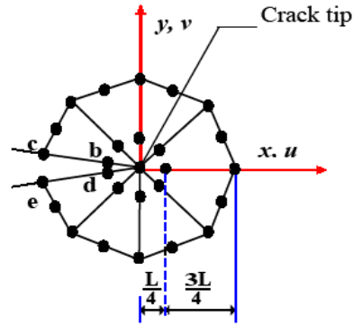
Figure 1: Singular element proposed by Barsoum, used for DET
