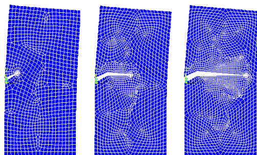
Figure 6: Crack propagation path of the inclined crack
