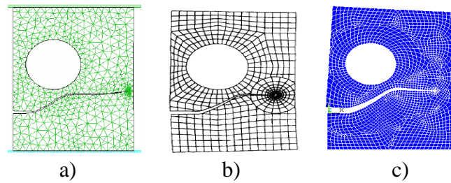
Figure 9: Final configuration corresponding to the last position of crack-tip (with E_2/E_1=1 ): a) Bouchard et al. [20], b) Rashid [21] and c) Present study
