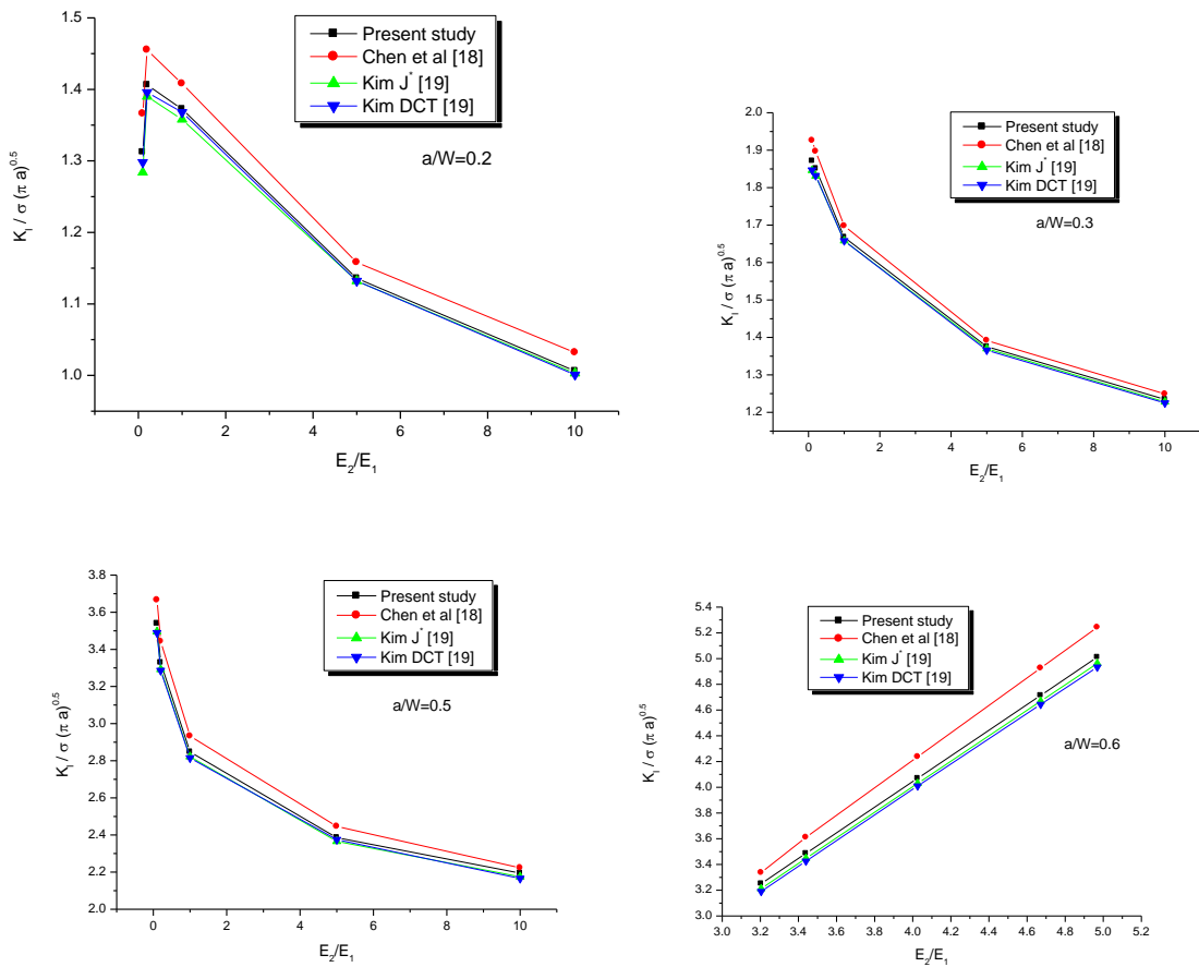
Figure 4: Normalized SIFs for edge cracked FGM plate for : a/w = 0.2, 0.3, 0.5 and 0.6
